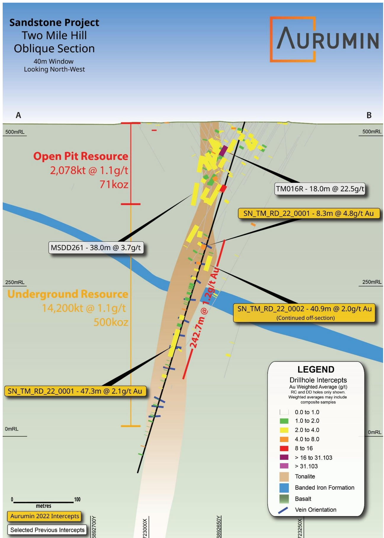
Figure 1- Oblique Section showing SN_TM_RD_22_0001
